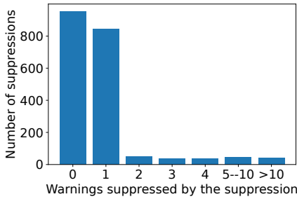
(a) Number of warnings suppressed by a single suppression.
