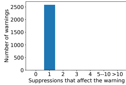
(b) Number of suppressions that affect a single warning.
